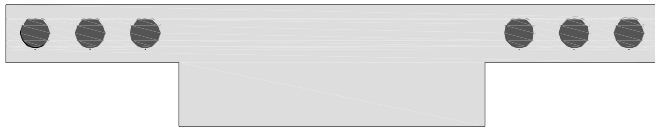
Rear T-Bar with (6) 4 in. Round Light Holes IC975003-14
